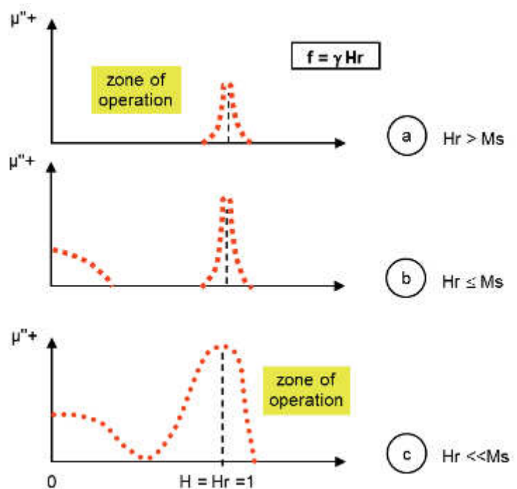
Figure 2 : permeability \mu''_+ versus static field H
